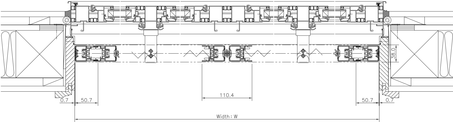
Caterpillar2 Double door (88LW) Cross section
