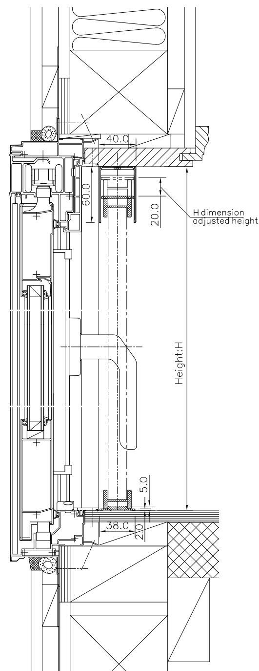
Caterpillar2 (88LW) Longitudinal section
