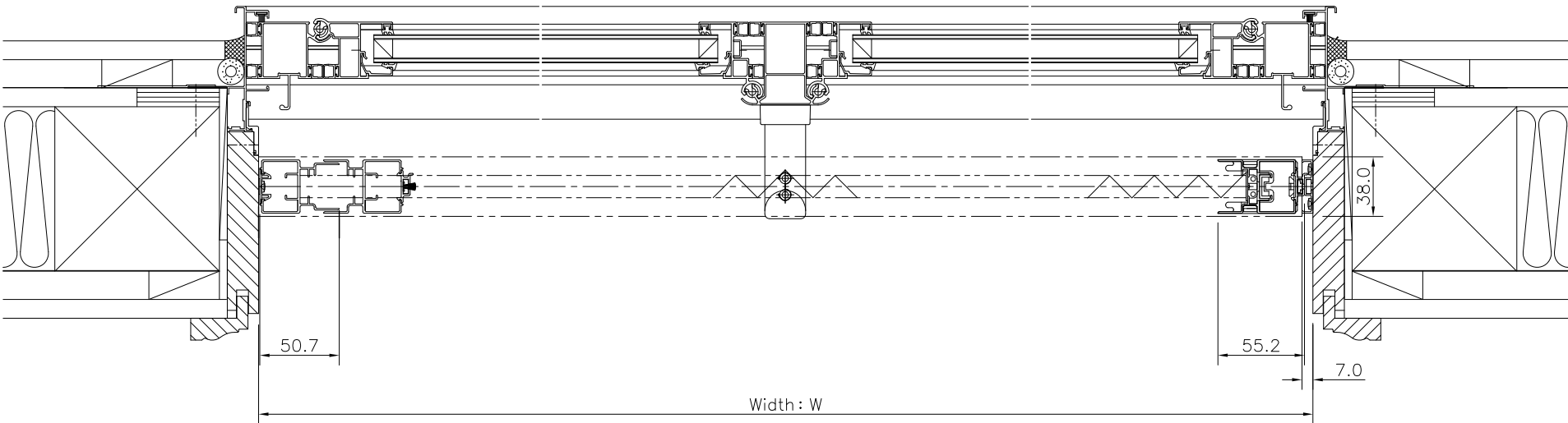
Caterpillar2 Single door (88LW) Cross section
