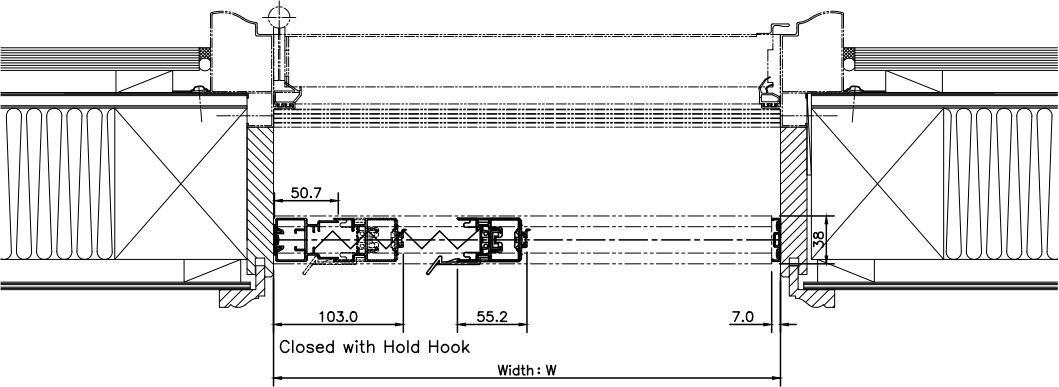
Caterpillar2 Single door (88L) Cross section
