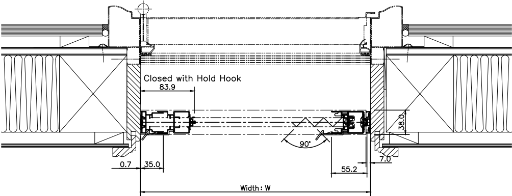
Caterpillar2 Single door (8LF) Cross section
