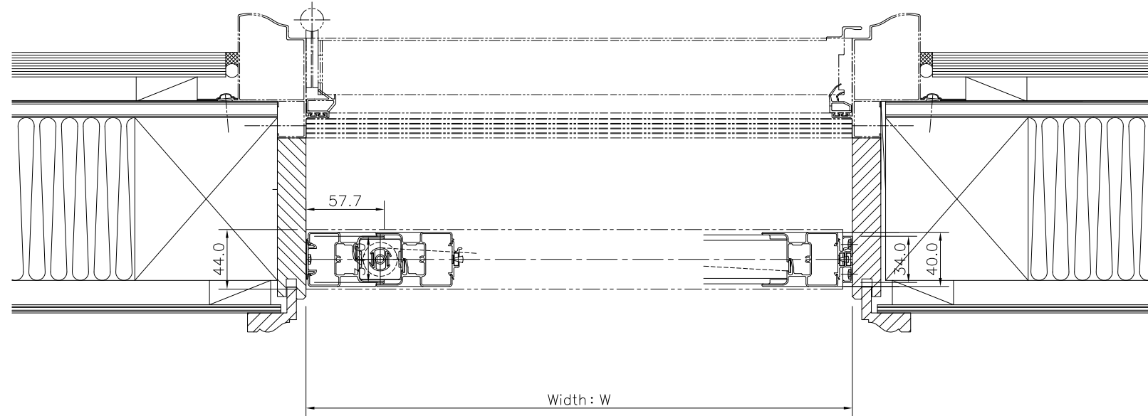
Single door Cross section
