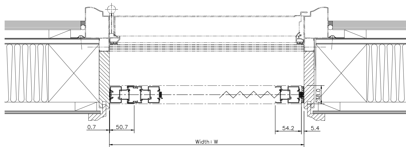
Zipooh Single door (88LME) Cross section
