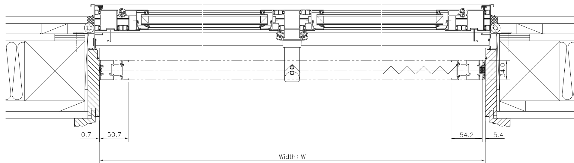
Zipooh Double door (88LMEW) Cross section
