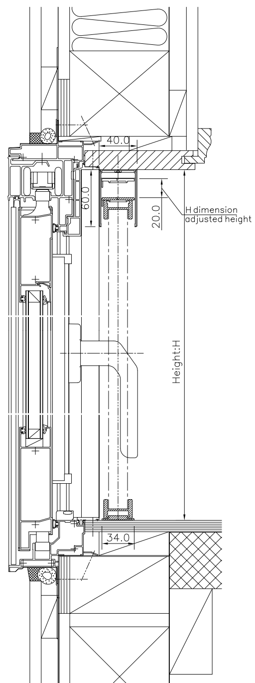
Zipooh (88LMEW) Longitudinal section
