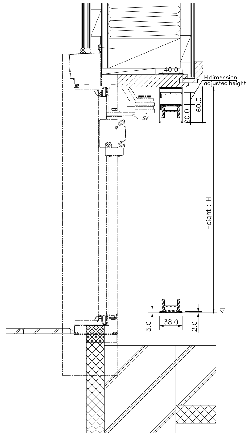
Zipooh Double door (8LME) Cross section
