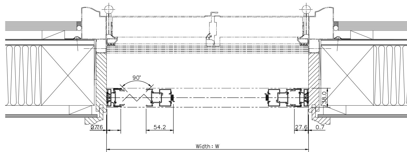
Zipooh Double door (8LME) Cross section
